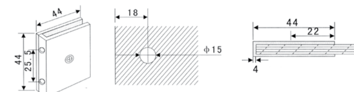
Spojnica zid - staklo, mala inox MAT debljina stakla 8/10/12 mm
